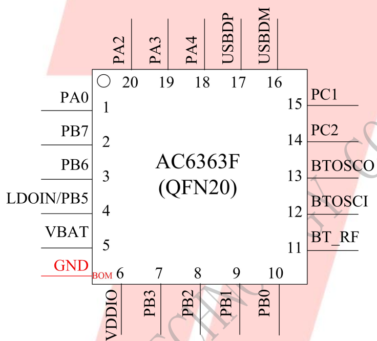
Figure 1-1 AC6363F Package Diagram
